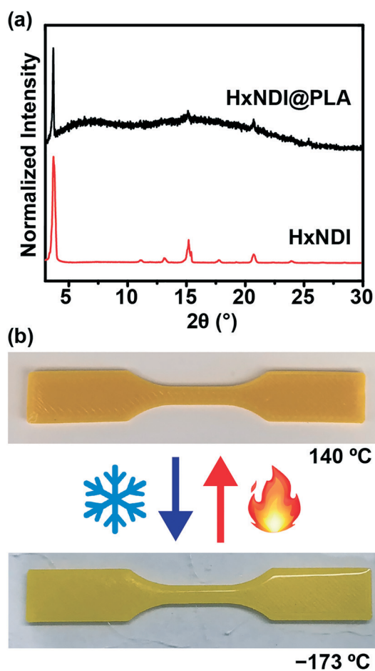
Fig. 7 (a) PXRD data for HxNDI@PLA composites and (b) positive thermochromic behavior of HxNDI @PLA.
