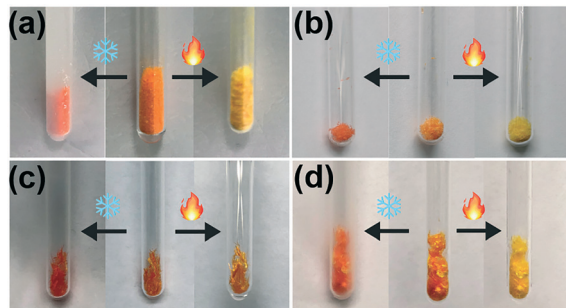
Fig. 5 Thermochromic behavior of (a) PNNDI, (b) HNNDI, (c) ONNDI, and (d) NNNDI. All the samples were heated to 100 °C and cooled to -173 °C for the visualization of thermochromic behavior.
