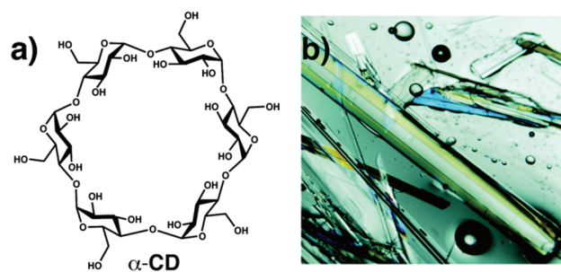
Figure 1. (a) Structural formula of \alpha -cyclodextrin ( \alpha -CD), a naturally occurring cyclic oligosaccharide comprised of six \alpha -1,4-D-Glucp residues portrayed in their stable {}^4\text{C}_1 conformations. (b) The strawlike crystals of CD-MCF obtained under controlled crystallization conditions, formed from the self-assembly of \alpha -CD and \text{Rb}^+ ions, contain inner pore diameters in the range of 100 nm to 2 mm.
