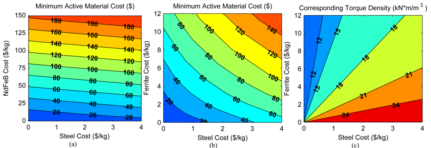
Fig. 17. Effect of Steel and Magnet Costs on (a) Minimum Active Material Cost of NdFeB Designs, (b) Minimum Active Material Cost of Ferrite Designs, and (c) the Corresponding Torque Density of the Minimum Active Material Cost Ferrite Designs
