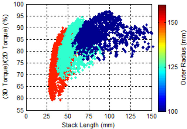
Fig. 8. Impact of Outer Radius on 3D Effects for NdFeB Gear Designs at Different Stack Lengths
