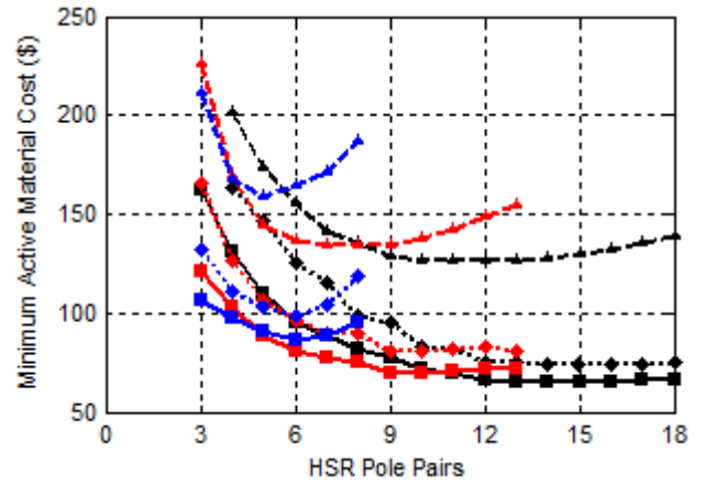
Fig. 13. Impact of HSR Pole Pairs on the Minimum Active Material Cost
