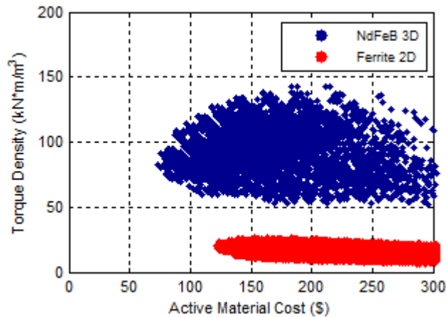
Fig. 5. Torque Density and Cost for the Best Designs based on 3D NdFeB and 2D Ferrite Simulations
