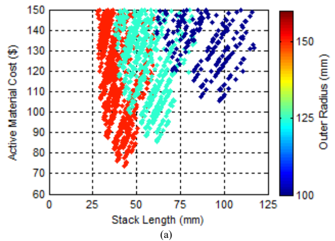
Fig. 6. Active Mass and Cost for the Best Designs based on 3D NdFeB and 2D Ferrite Simulations
