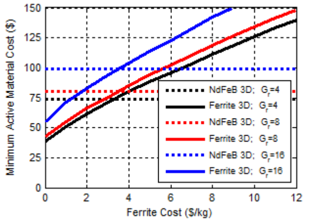
Fig. 16. Impact of Ferrite Cost Variation on Minimum Active Material Cost
