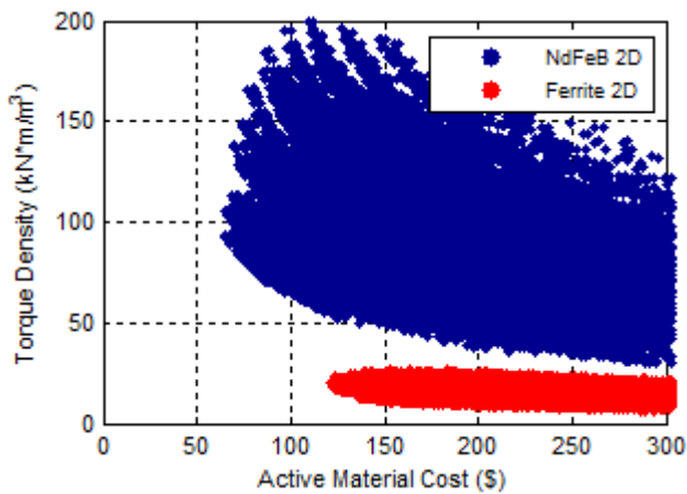
Fig. 3. Torque Density and Cost for the Best Designs based on 2D Simulations
