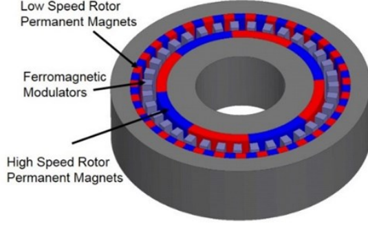
Fig. 2. Radial Flux Magnetic Gear with Surface Permanent Magnets
