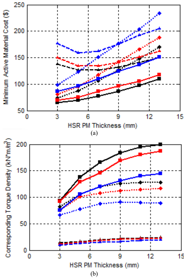
Fig. 12. Impact of HSR Magnet Thickness on (a) the Minimum Active Material Cost and (b) the Corresponding Torque Density
