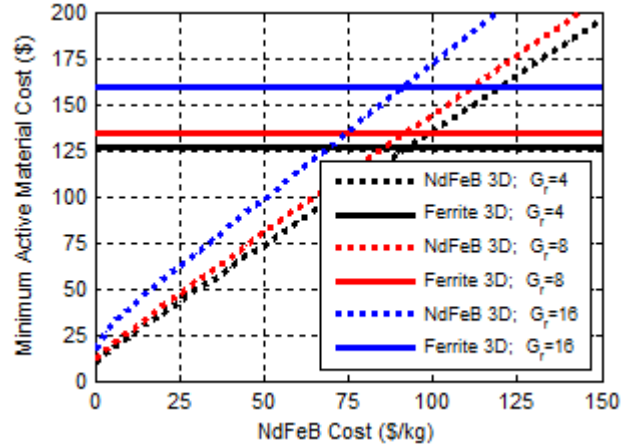
Fig. 15. Impact of NdFeB Cost Variation on Minimum Active Material Cost
