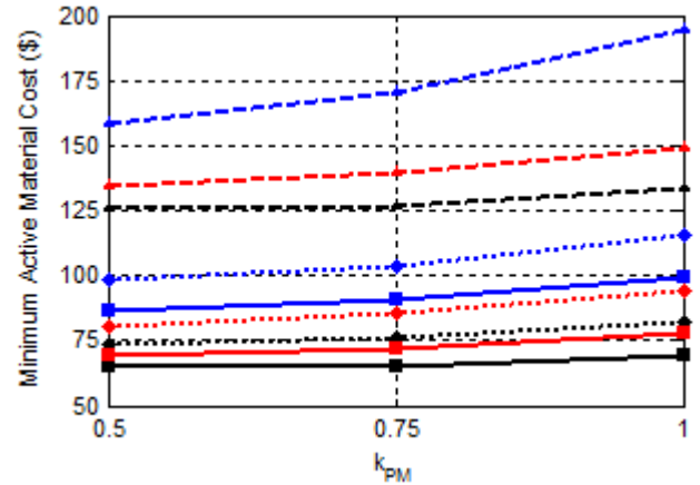
Fig. 14. Impact of k_{PM} on the Minimum Active Material Cost
