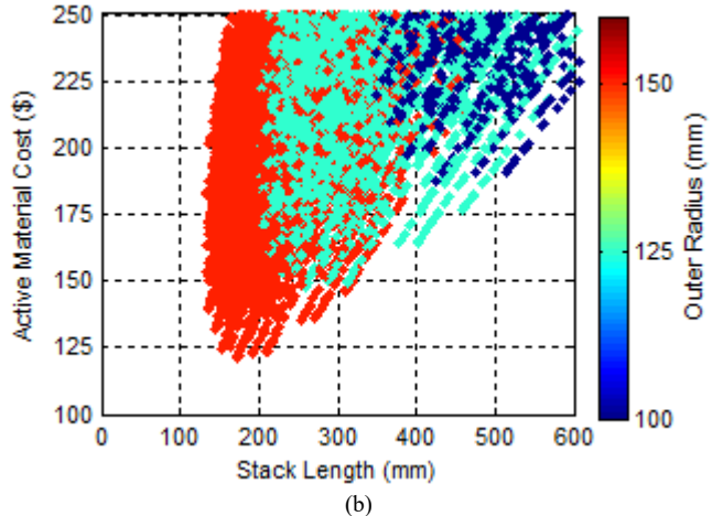
Fig. 7. Relationship between Stack Length, Active Material Cost, and Outer Radius for (a) 3D NdFeB and (b) 2D Ferrite Magnetic Gear Simulations
