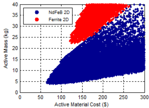
Fig. 4. Active Mass and Cost for the Best Designs based on 2D Simulations
