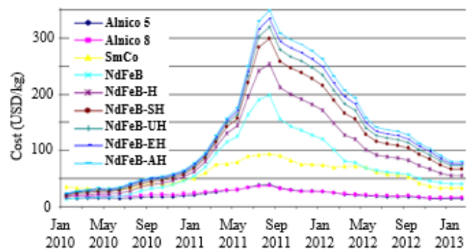
Fig. 1. Rare Earth Permanent Magnet Cost Trends [12].
