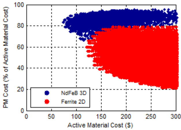
Fig. 10. Percentage of Total Active Material Cost from Magnet Material for NdFeB and Ferrite Designs
