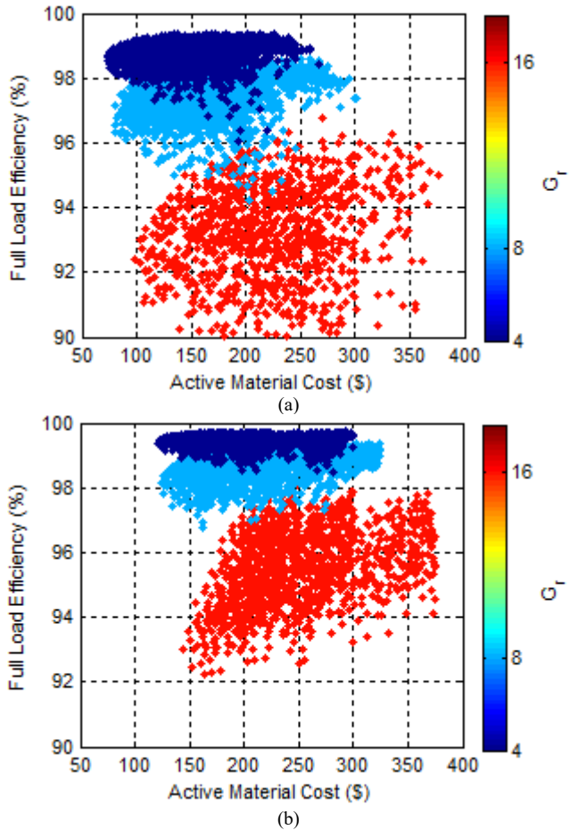
Fig. 9. Efficiencies for the Best (a) NdFeB and (b) Ferrite Gear Designs
