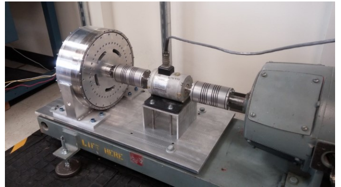
Fig. 12. AFMGM Prototype on Testbed
