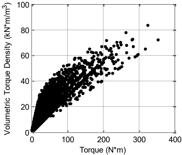
Fig. 7. Volumetric Torque Density vs. Torque Rating
