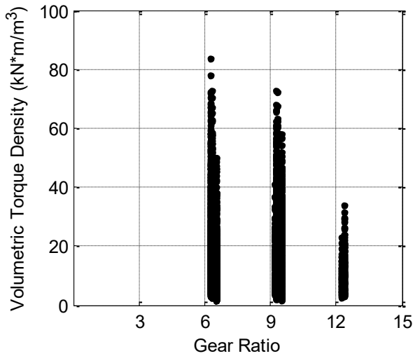
Fig. 6. Volumetric Torque Density vs. Gear Ratio
