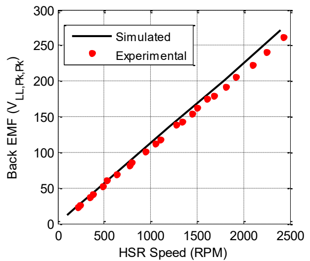
Fig. 15. Experimental and Simulated AFMGM No Load Back EMF Amplitude Characteristics
