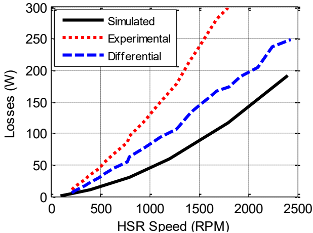
Fig. 17. Experimental and Simulated No Load AFMGM Losses
