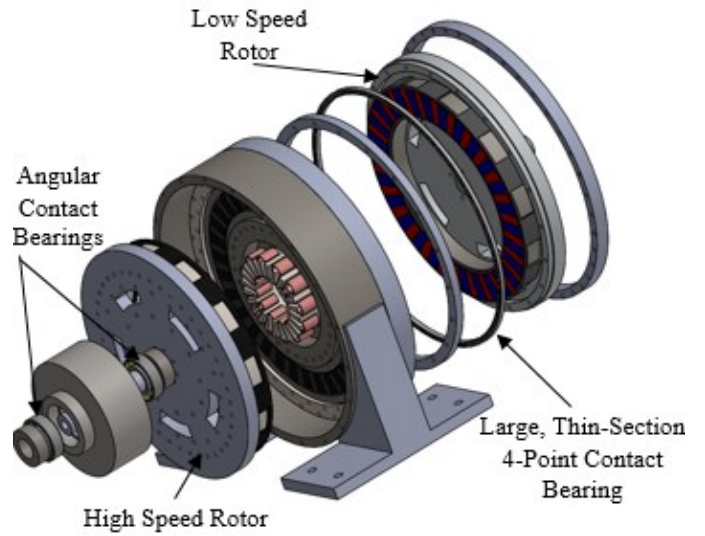
Fig. 11. Exploded View of AFMGM Prototype
