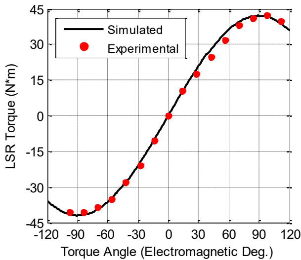
Fig. 13. AFMGM Prototype LSR Static Torque Characteristics Curve
