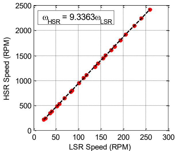
Fig. 14. AFMGM Prototype Gear Ratio Measurements
