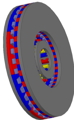
Fig. 3. Proposed Compact Axial Flux Magnetically Geared Machine Topology
