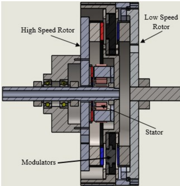
Fig. 10. Cutaway View of AFMGM Prototype
