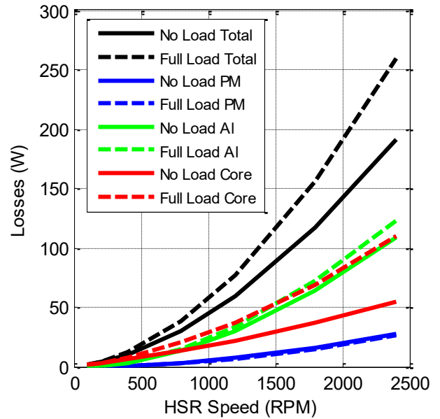
Fig. 18. Simulated No Load and Full Load Magnetic Loss Components
