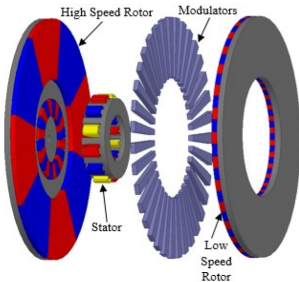
Fig. 4. Exploded View of the Proposed Compact AFMGM
