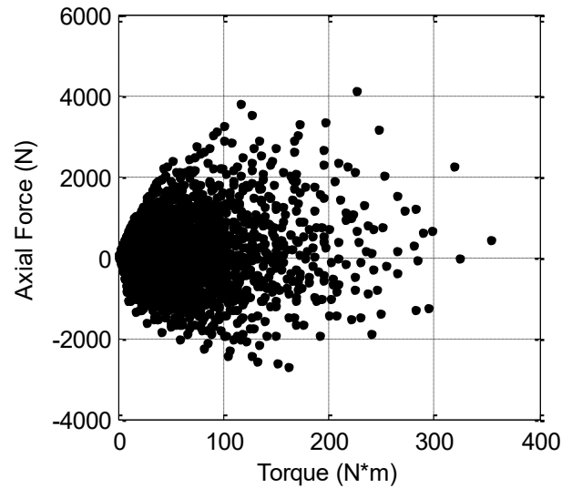
Fig. 9. Total Axial Forces on Modulators vs. Torque Rating
