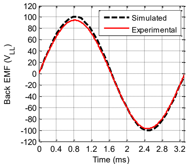
Fig. 16. Simulated and Experimental No Load Back EMF Waveforms at an HSR Speed of 1800 rpm
