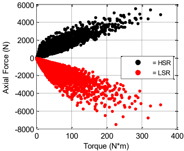
Fig. 8. Axial Forces on Rotors vs. Torque Rating
